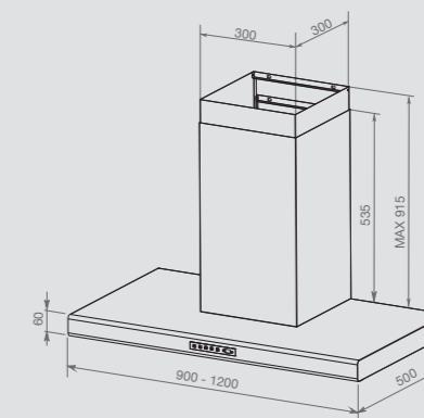
Technical drawing (cm):
