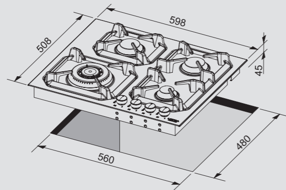
Technical drawing (cm):
