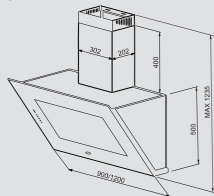
Technical drawing (cm):
